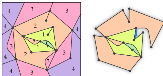
FIGURE 4. The left figure shows a portion of an infinite planar map with faces coloured according to (dual) graph distance to the root-face. The sub-map on the right depicts a possible state of the peeling by layers. Its hole has three edges at height h = 1 and eleven edges at height h + 1 = 2 . The next peel edge is indicated in blue.
