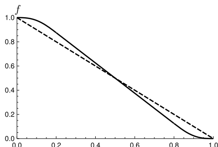
FIGURE 5. The solid curve corresponds to a function f satisfying the hypotheses of Lemma 6 with \varepsilon = 0.2 , while the dashed lined depicts x \mapsto 1 - x .
