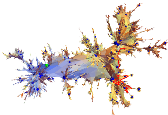
FIGURE 1. A representation of a geodesic ball in a randomly sampled infinite map considered in this paper. The blue balls indicate high degree vertices, the green ball is the root-vertex, while the red curve indicates the boundary of the ball.
