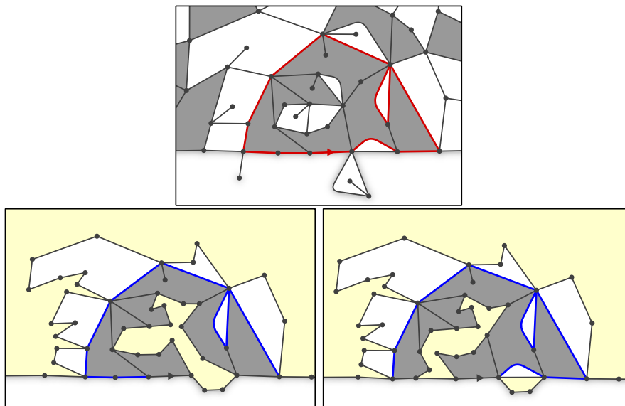
FIGURE 8. Illustration of the outer-most boundary of the percolation cluster: \mathcal{L} = 12 is the number of edges on the red cycle and \mathcal{N} = 9 and \mathcal{N}' = 9 are the number of edges on the blue path on the left and on the right respectively.
